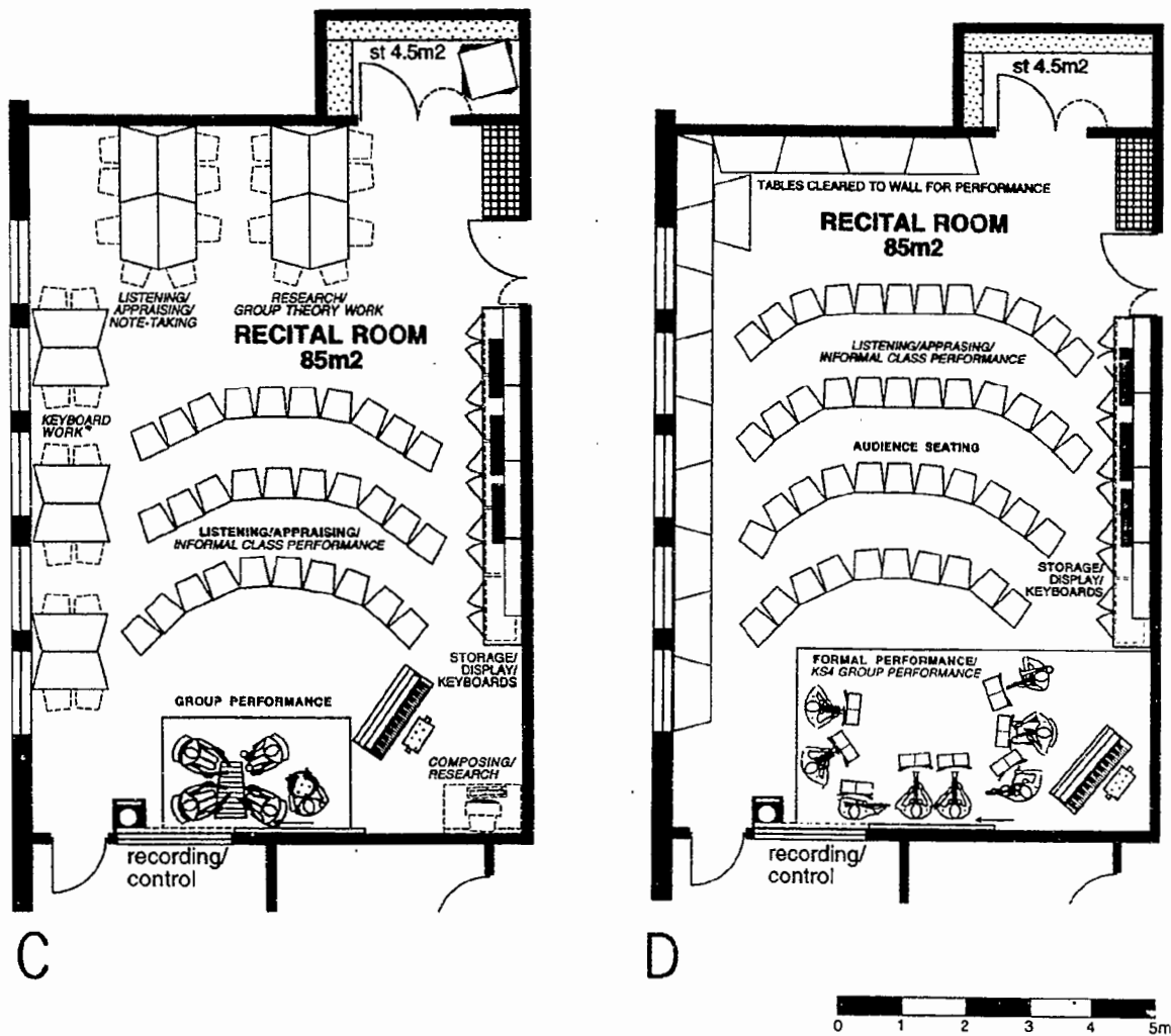
Figure 2/4 C & D 85m² music class/recital room planned for a range of activities
