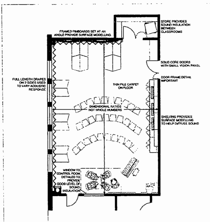
Figure 4/9 Acoustic treatment to music class/recital room
