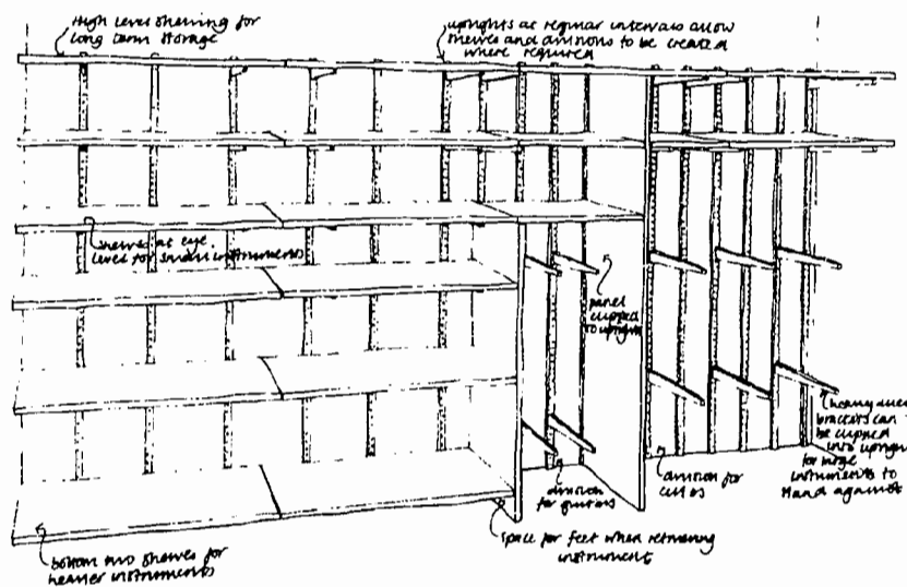
Figure 3/5 Instrument store: adjustable shelving system (700mm deep shelves)
