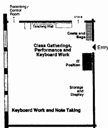
Figure 2/2 Zoning diagram layout for a music classroom
