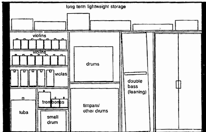
View A: 900mm deep shelving
