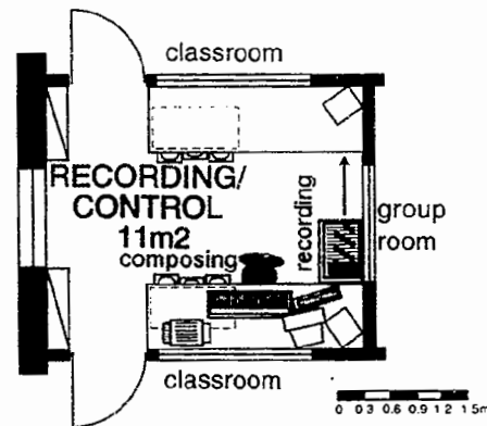
Figure 2/9 Recording/control room layout
