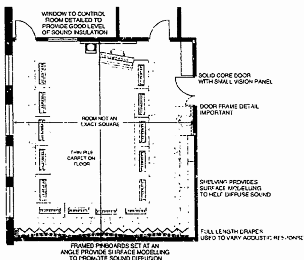
Figure 4/8 Acoustic treatment to music classroom
