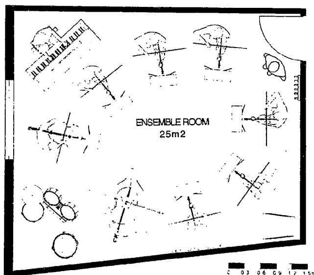
Figure 2/8 25m² ensemble room
