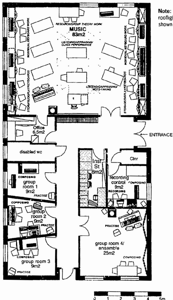
Figure 5/5 Case Study 2: the furnished plan
