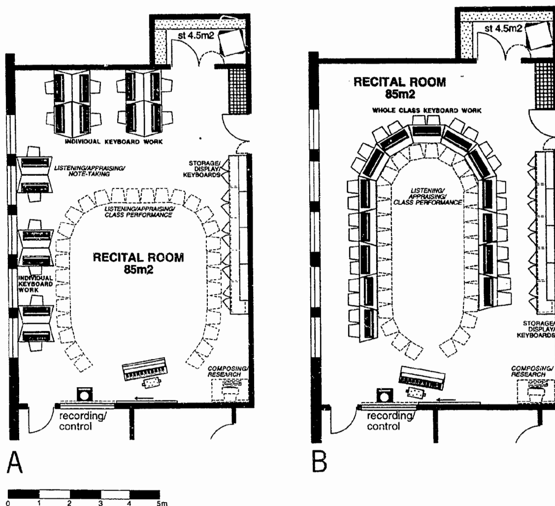
Figure 2/4 A & B 85m² music class/recital room planned for a range of activities
