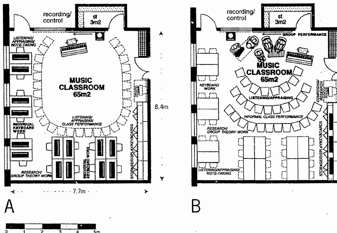
Figure 2/3 A & B 65m² music classroom planned for a range of activities
