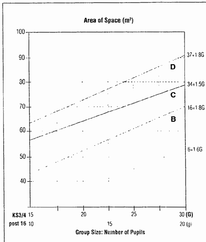
Figure 1/2 Area range for music according to group size
