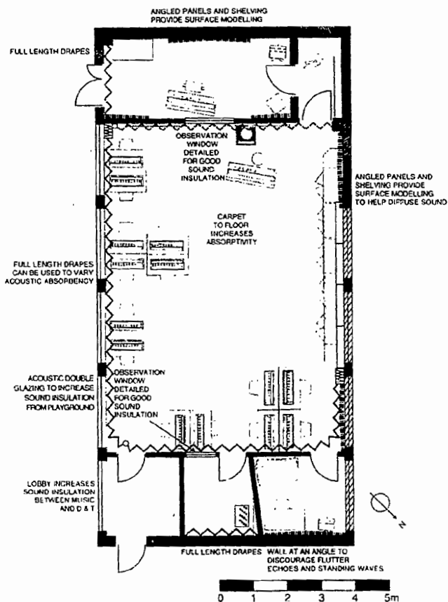
Figure 5/2 Case Study 1: acoustic treatment
